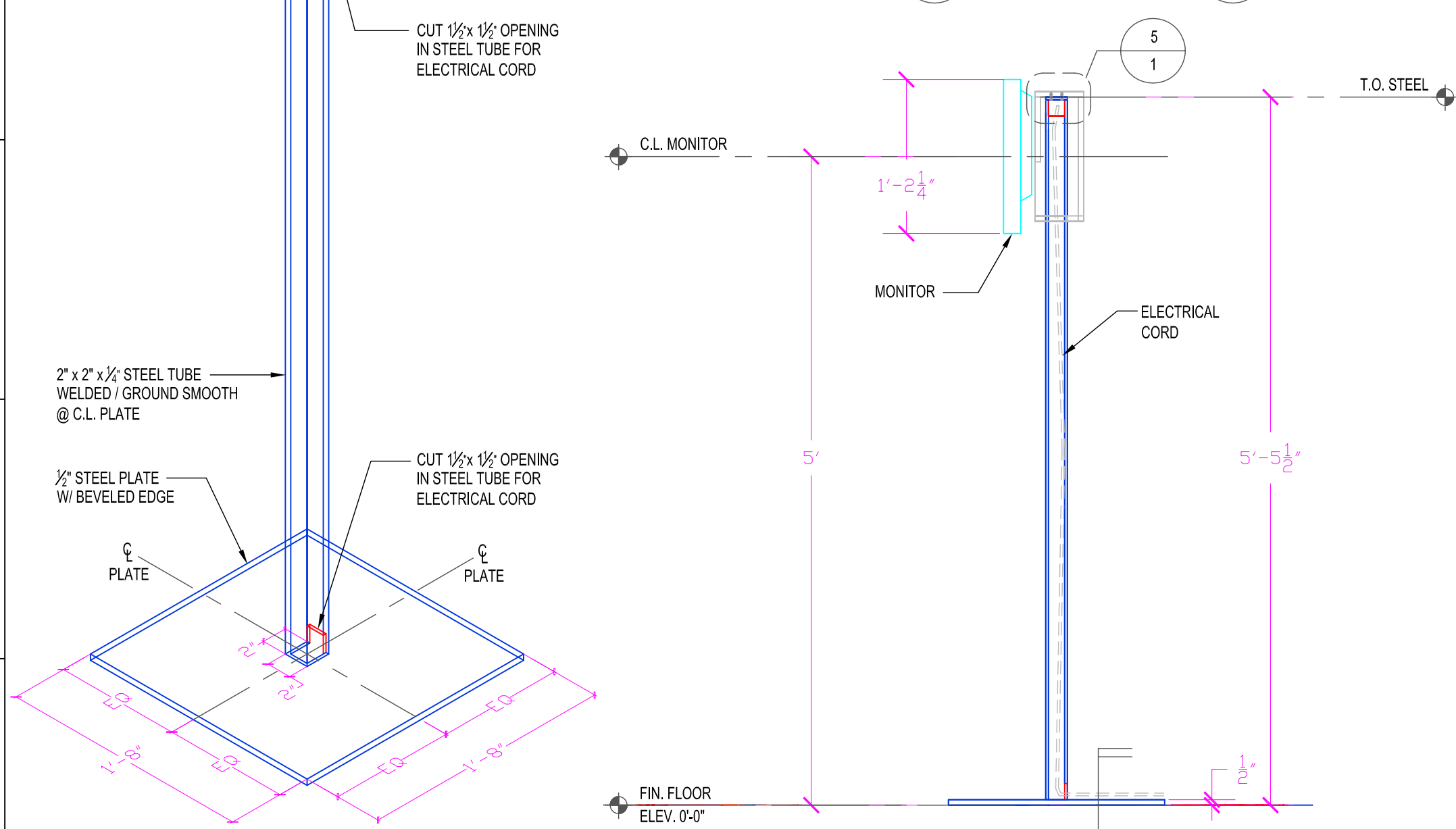
1 AXONOMETRIC VIEW @ STAND AND PLYWOOD CASE 1 SCALE: NTS
