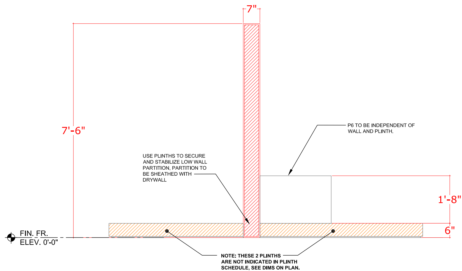
3 SECTION @ LOW WALL AND PLATFORMS SCALE: 3/4" = 1'-0"
