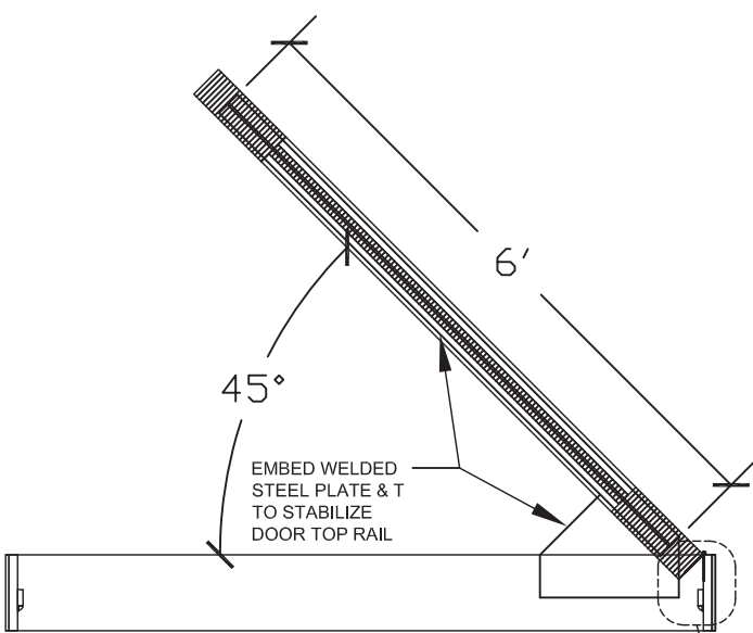
2 PLAN DOOR SWING SCALE: 1/2" = 1'-0"
